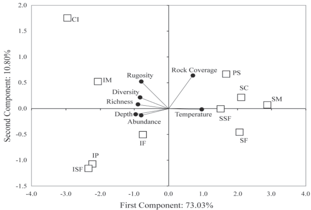
Figure 5. Principal component analysis of variables. IM = intermediate Melón, SM = shallow Melón, IP = intermediate Pardino, SP = shallow Pardino, IF= intermediate Faro, SF = shallow Faro, ISF = intermediate San Francisquito, SSF = shallow San Francisquito. Also shown the projections of variables; rock coverage, temperature, rugosity, richness species, abundance, and diversity of the sampling locations.
